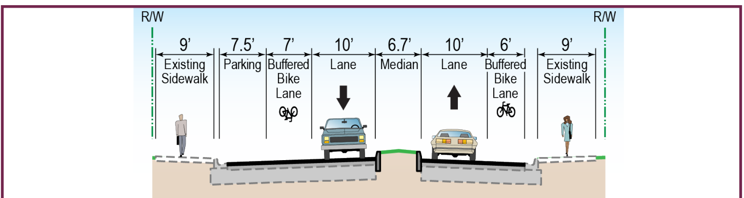
PROPOSED TYPICAL SECTION NO. 2 (SE 16TH STREET TO SE 15TH STREET) FACING NORTH
