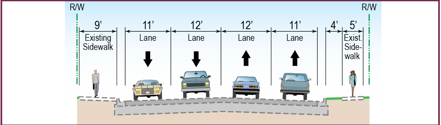
EXISTING TYPICAL SECTION NO. 1 (SE 17TH STREET TO SE 16TH STREET) FACING NORTH
