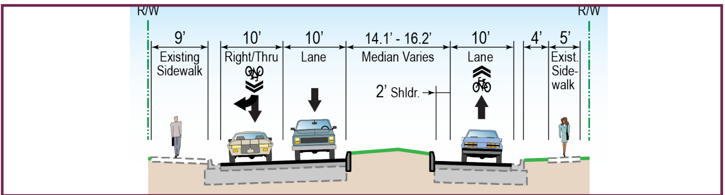
PROPOSED TYPICAL SECTION NO. 1 (SE 17TH STREET TO SE 16TH STREET) FACING NORTH
