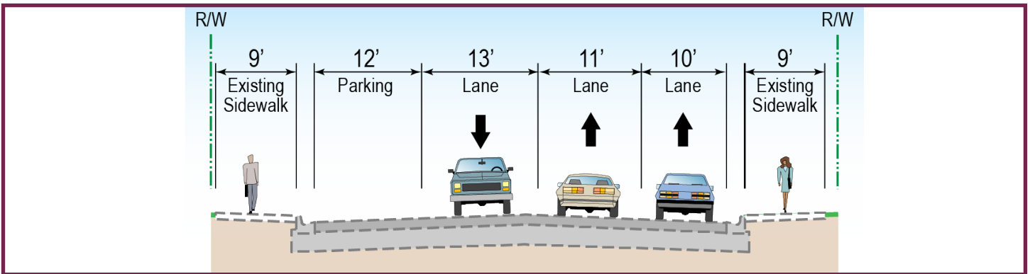
EXISTING TYPICAL SECTION NO. 2 (SE 16TH STREET TO SE 15TH STREET) FACING NORTH
